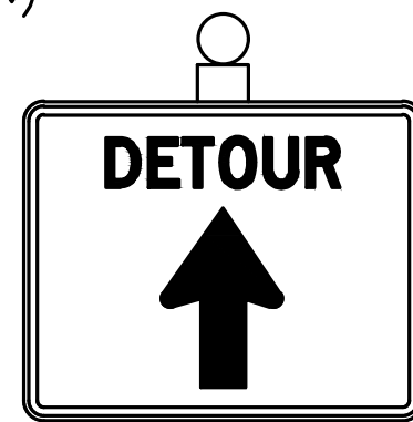
M4-9 (UP) BLACK ON ORANGE 30" X 24"
