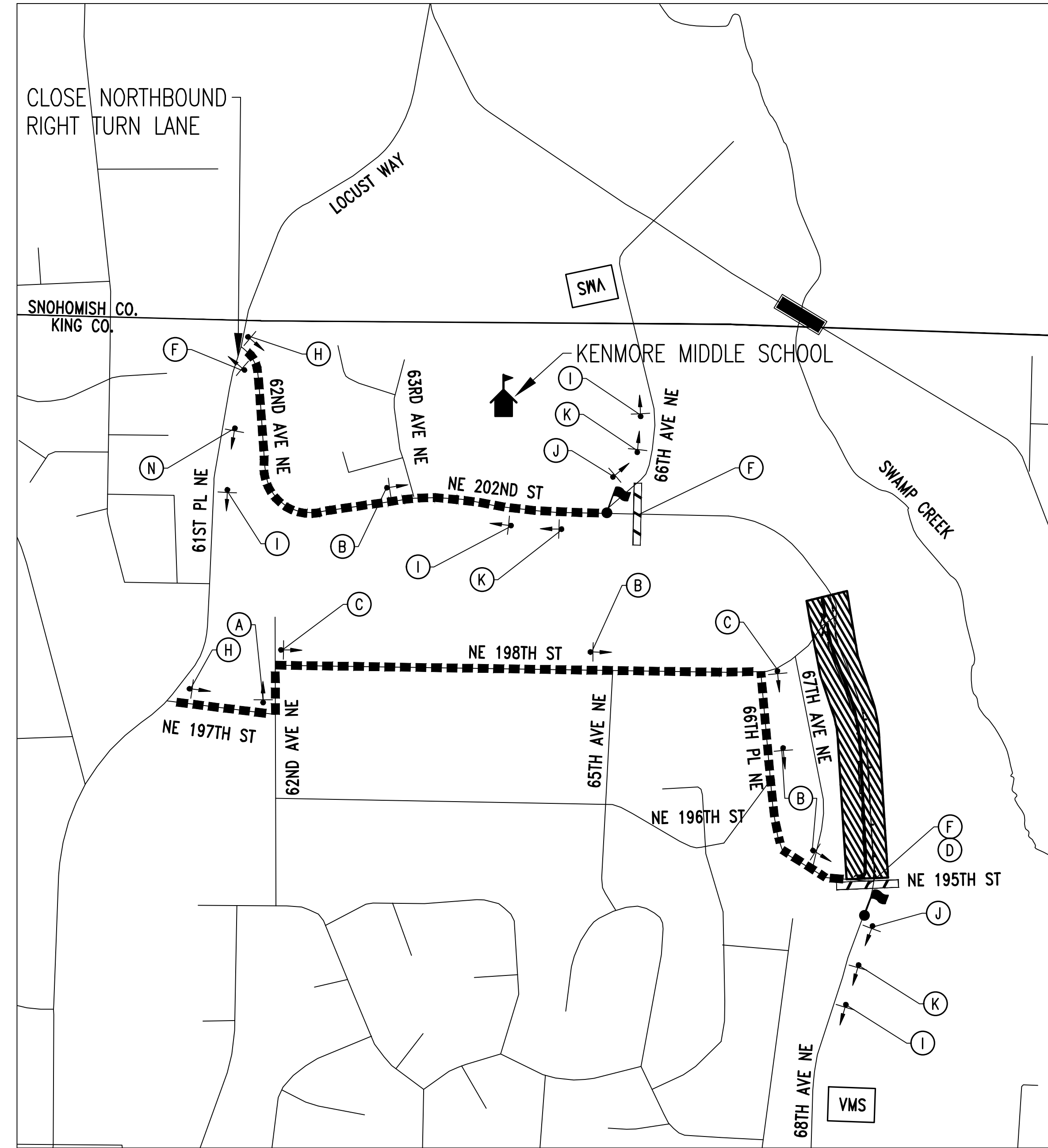
SEGMENT 3 NTS
