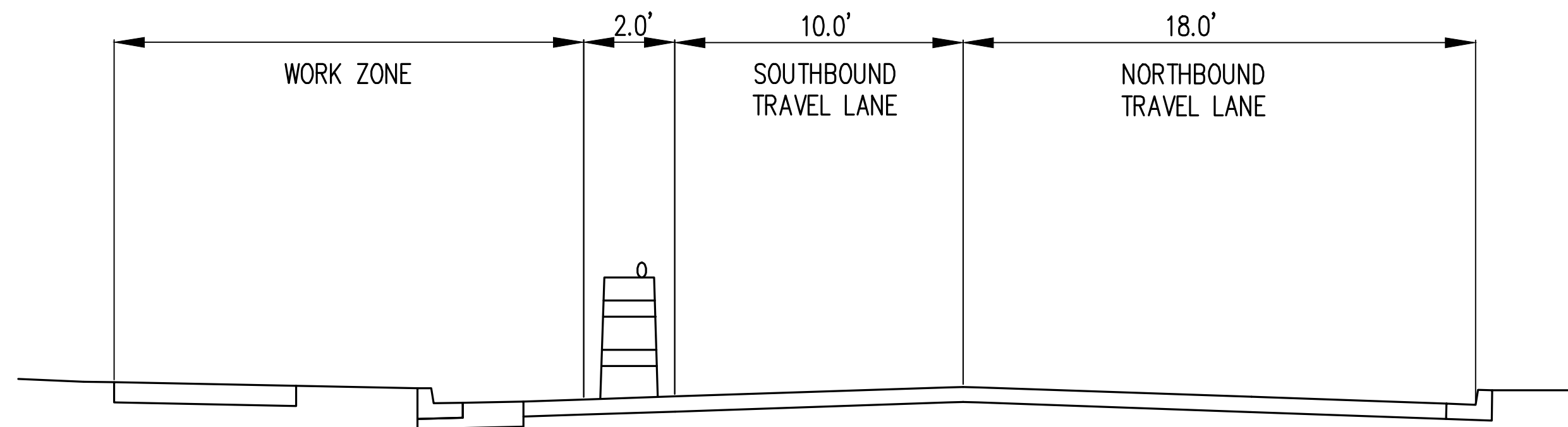
TRAFFIC CONTROL SECTION A
