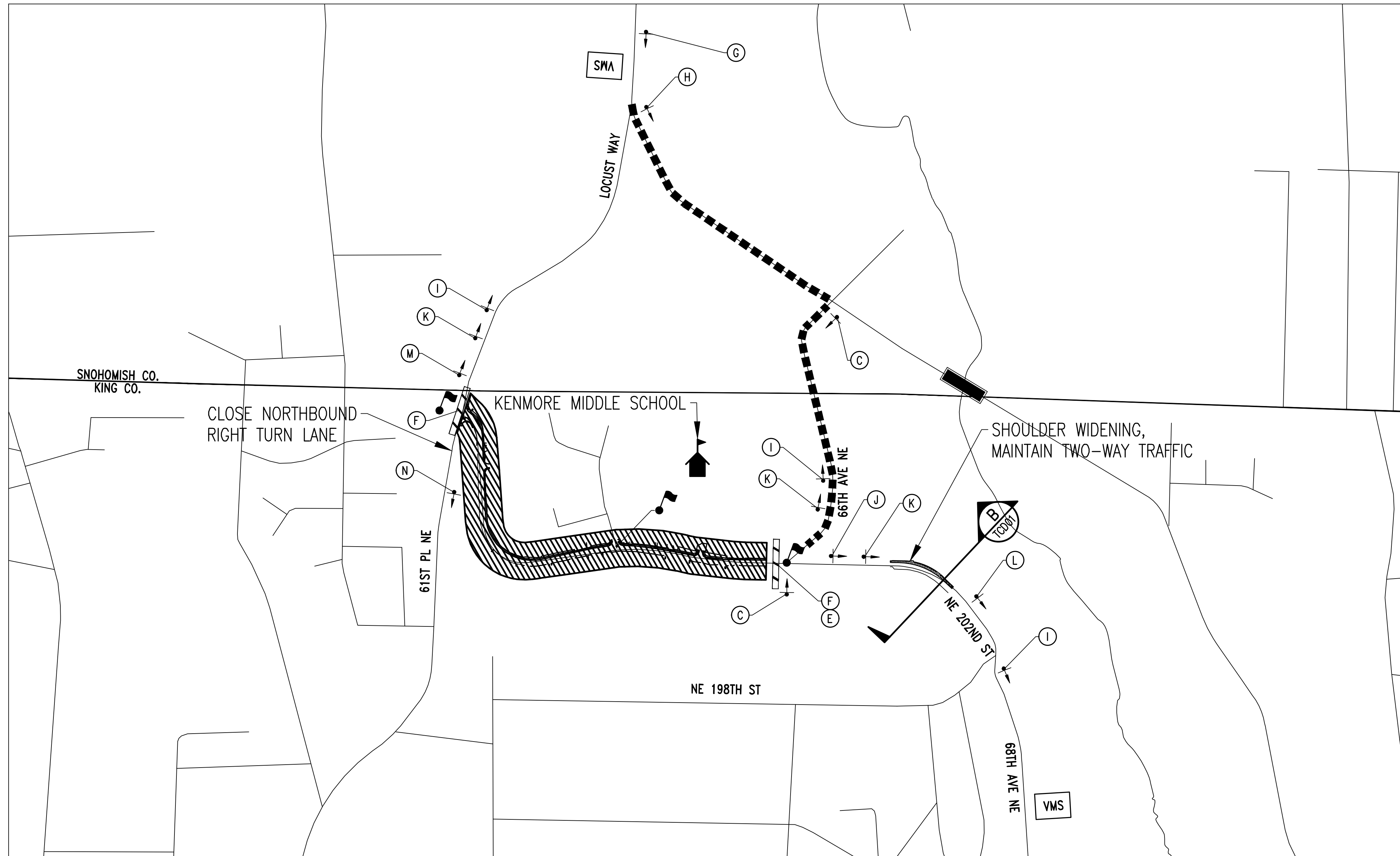
SEGMENT 4 NTS
