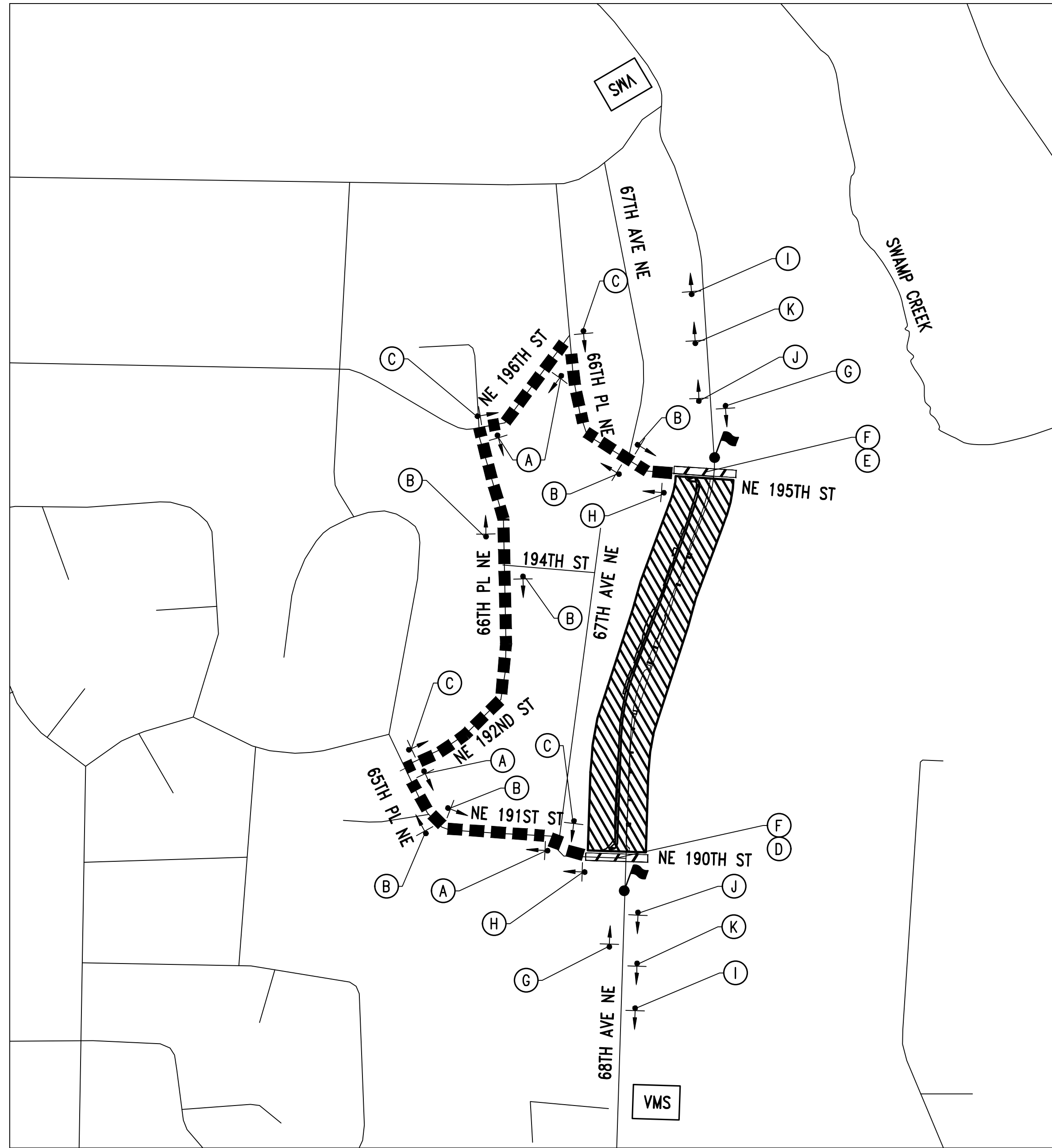
SEGMENT 2 NTS
