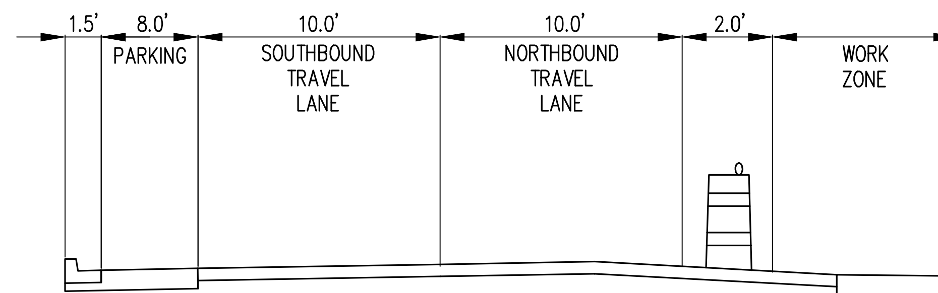
TRAFFIC CONTROL SECTION B
